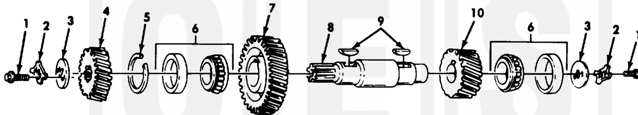
Figure 146. Transfer Intermediate Shaft and Related Parts.
